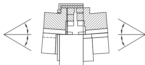
Angular Misalignment
