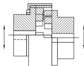
Radial Misalignment
